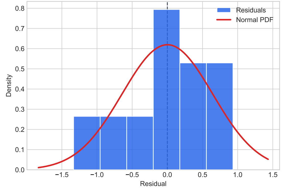
Residual Distribution
