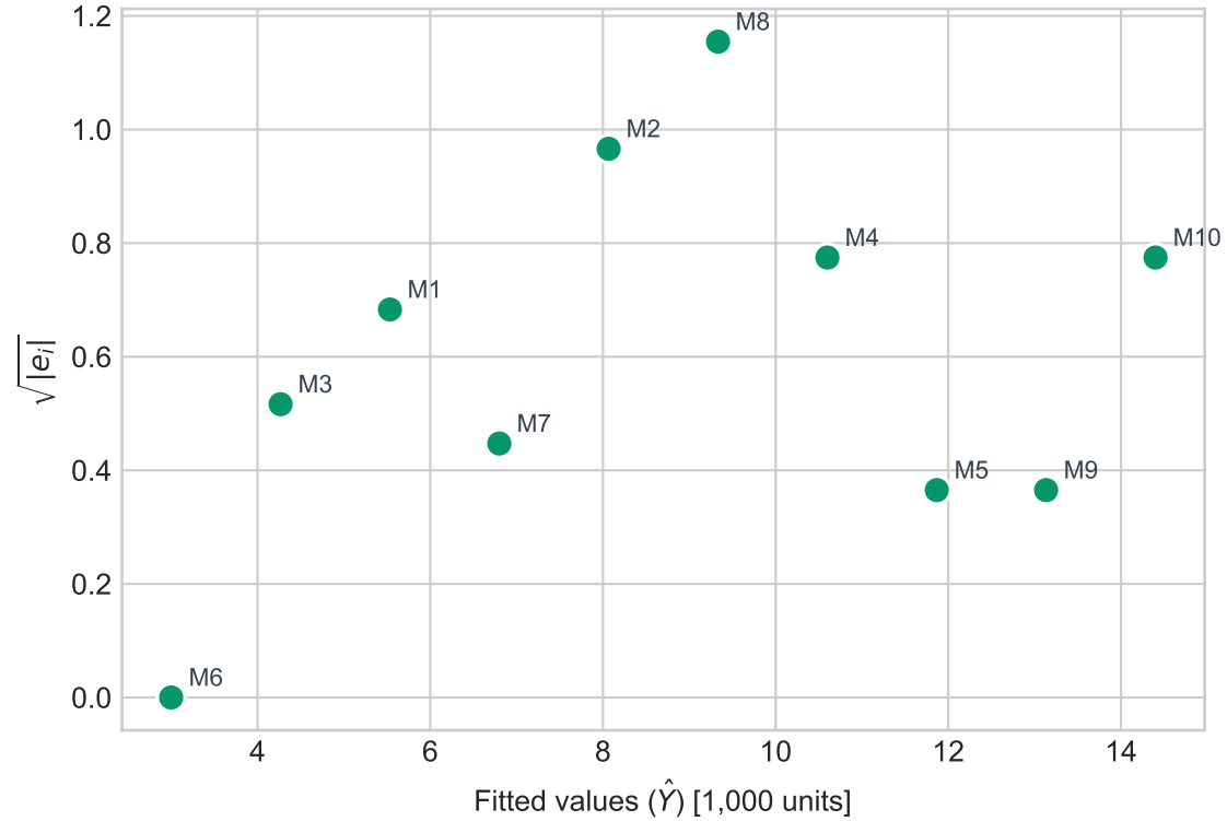
Scale-Location
