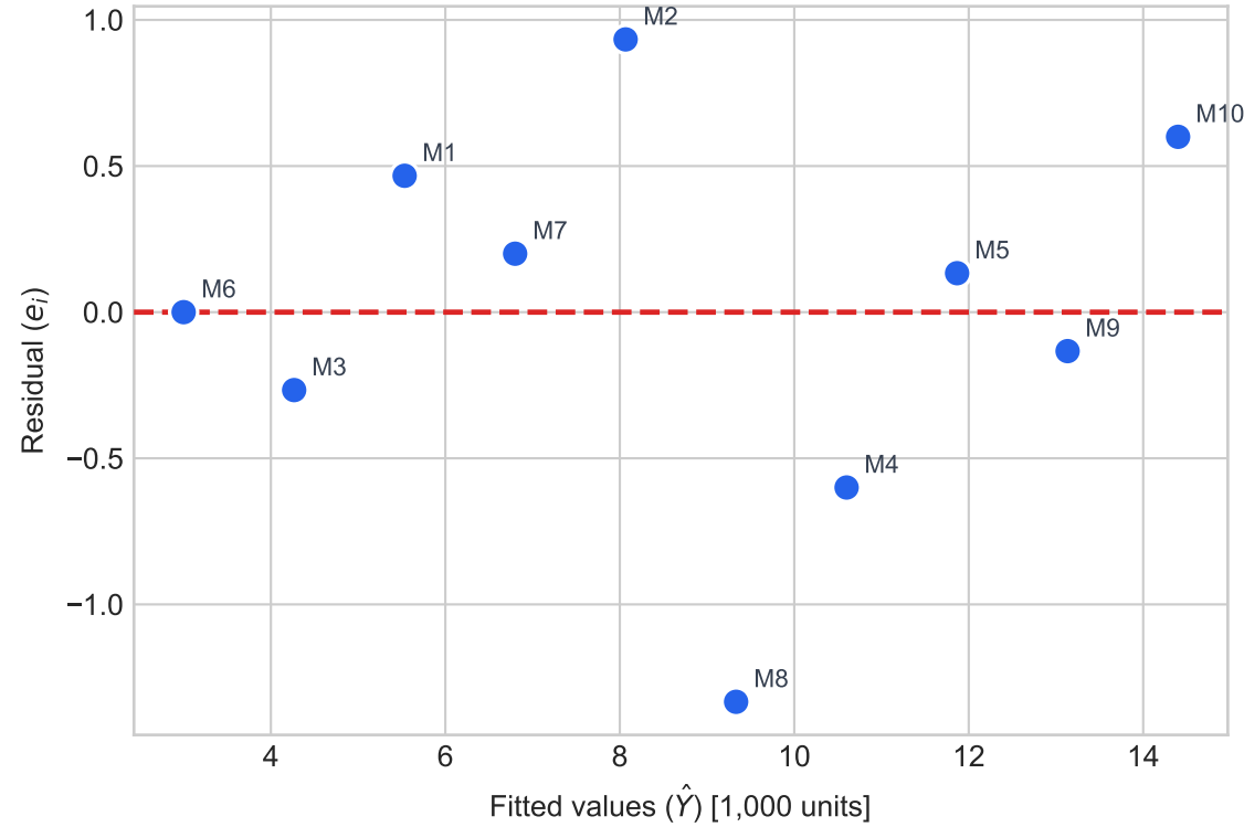
Residuals vs Fitted Values
